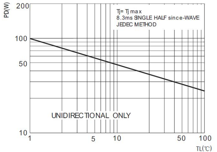
FIG6: Steady State Power Dissipation
